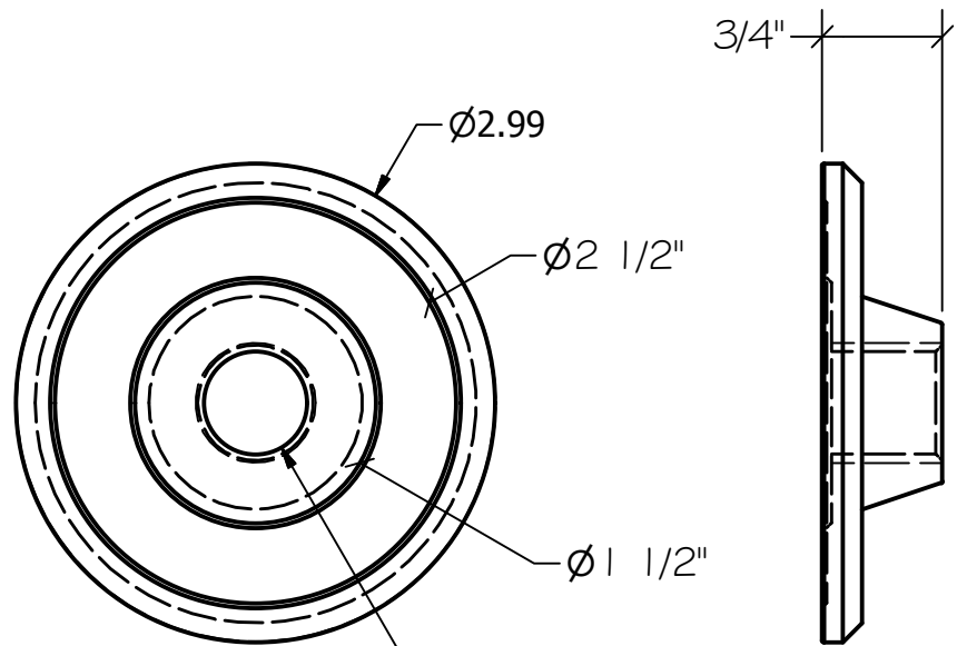
844-2 3/4-10 UNC - 2B x 3/4
